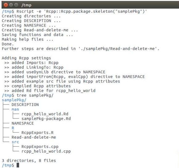
Fig. 3. Illustration of Rcpp::package.skeleton function.
